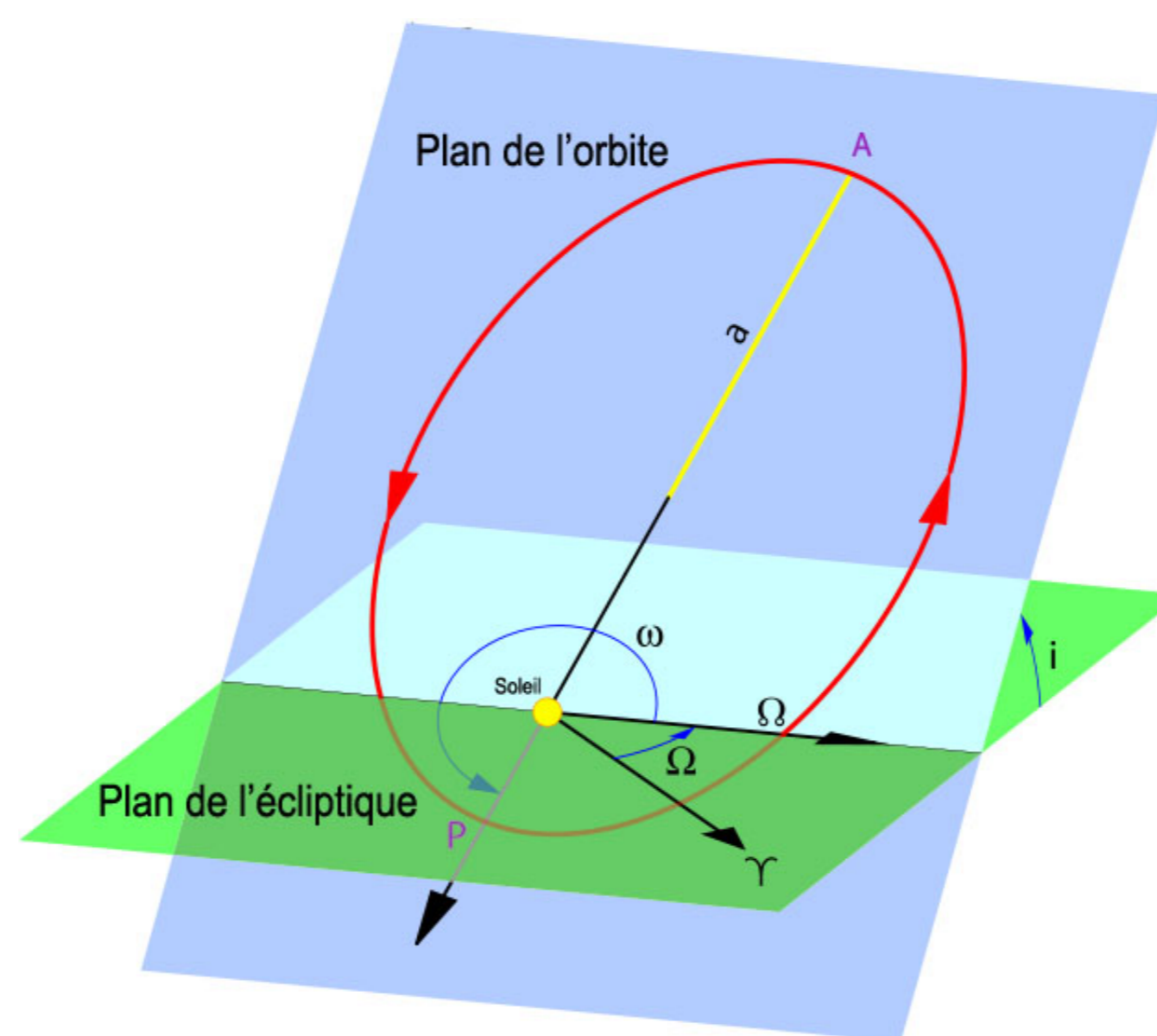
3d Planet Orbit Simulator
